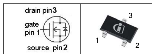
PG-SC-59
