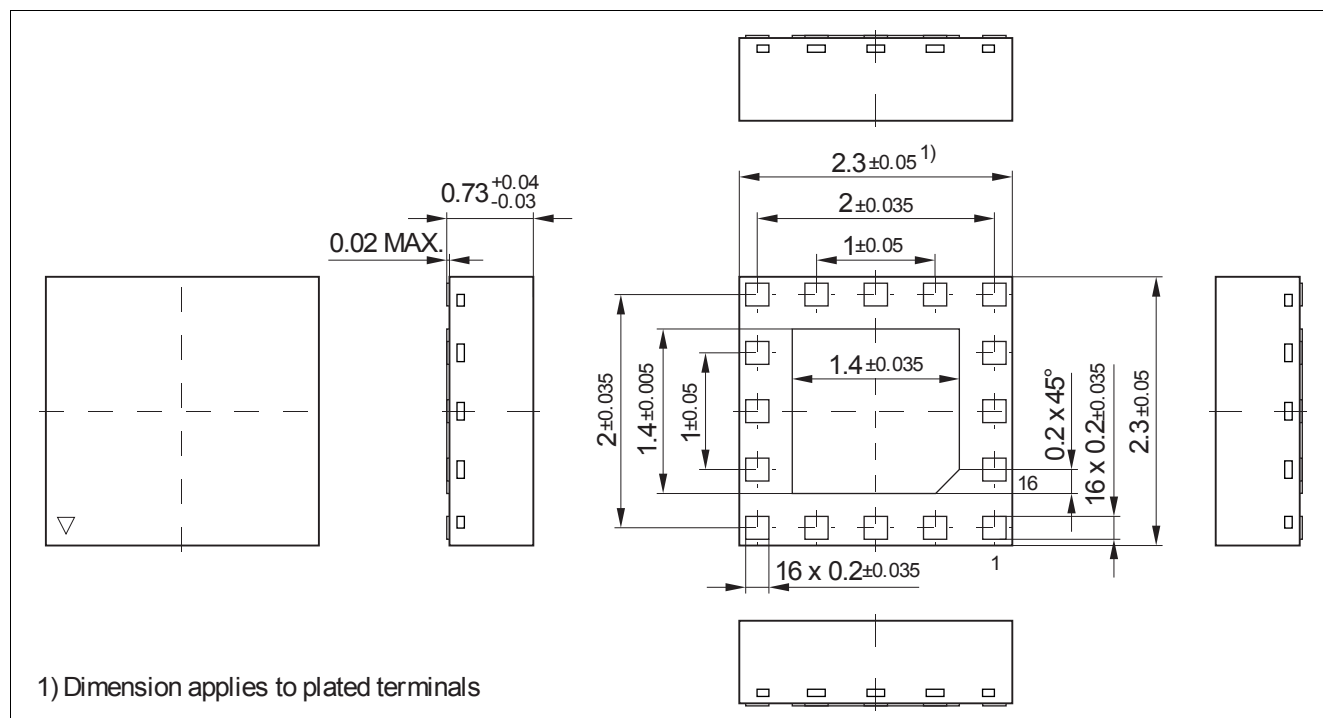
Figure 3 Package Outline
