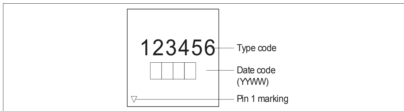
Figure 4 Pin Marking
