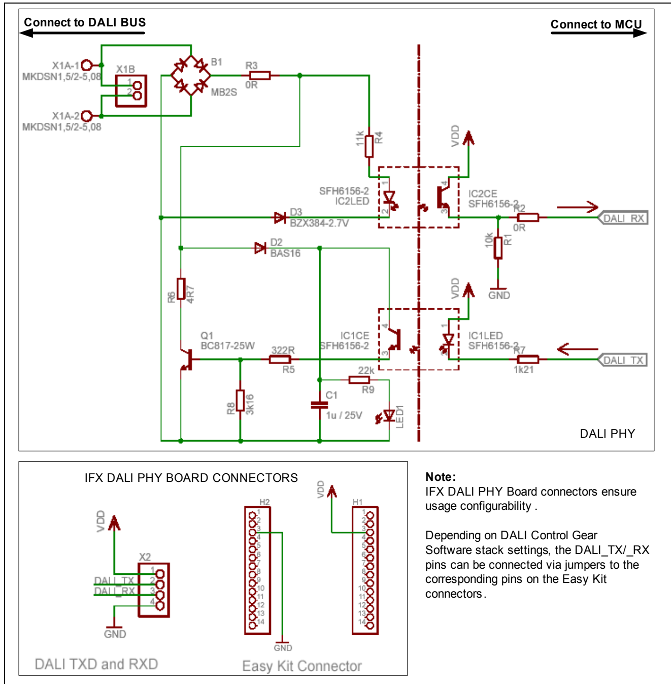
Figure 30 DALI PHY Board Schematics
