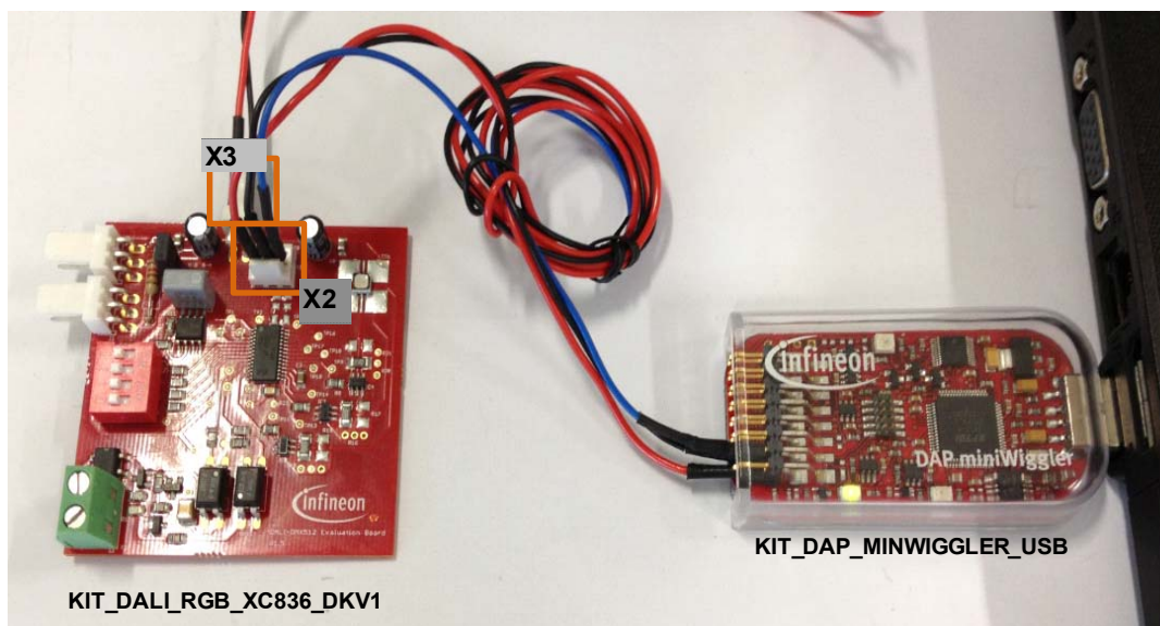
Figure 17 Programming the Control Gear using DAP miniWiggler
