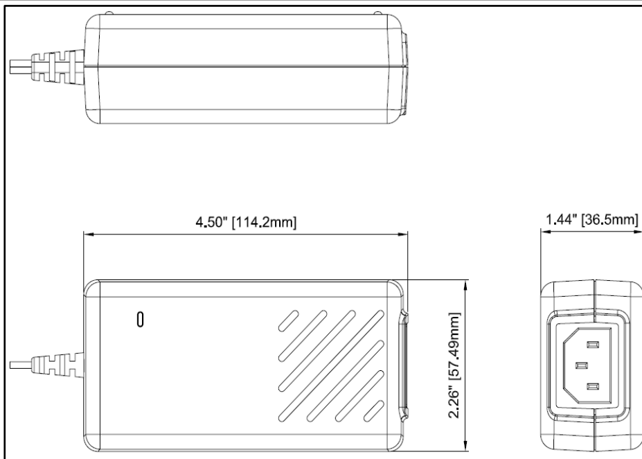
FWE050-Class I-DWG
