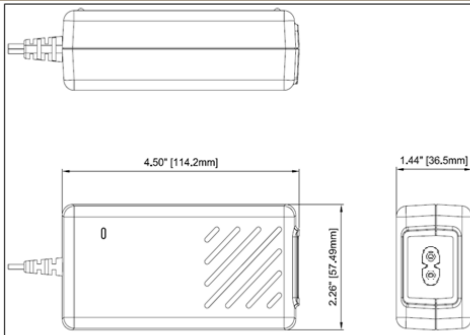
FWE050-DWG
