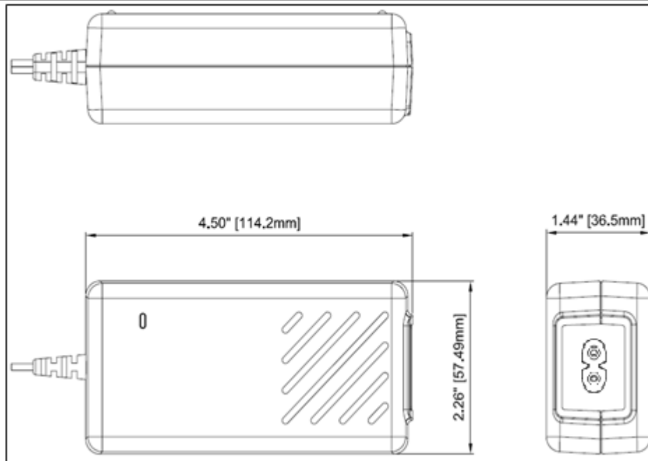
FWE050-Class II-DWG
