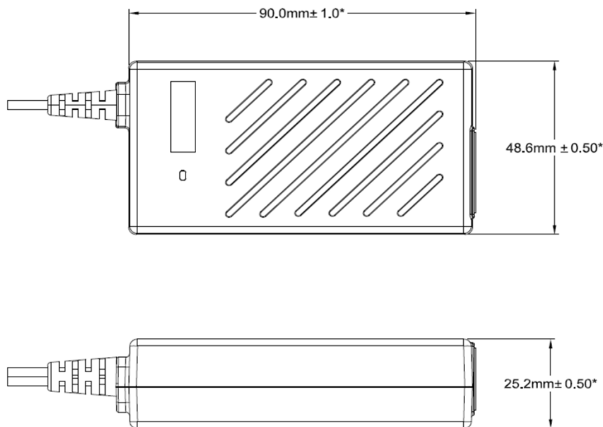
FWA020-Class I-DWG
