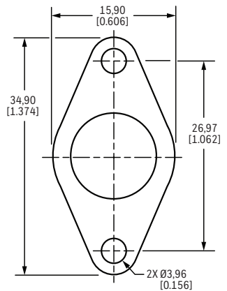
Figure 6. 3001/3004 Series Radius Cap
