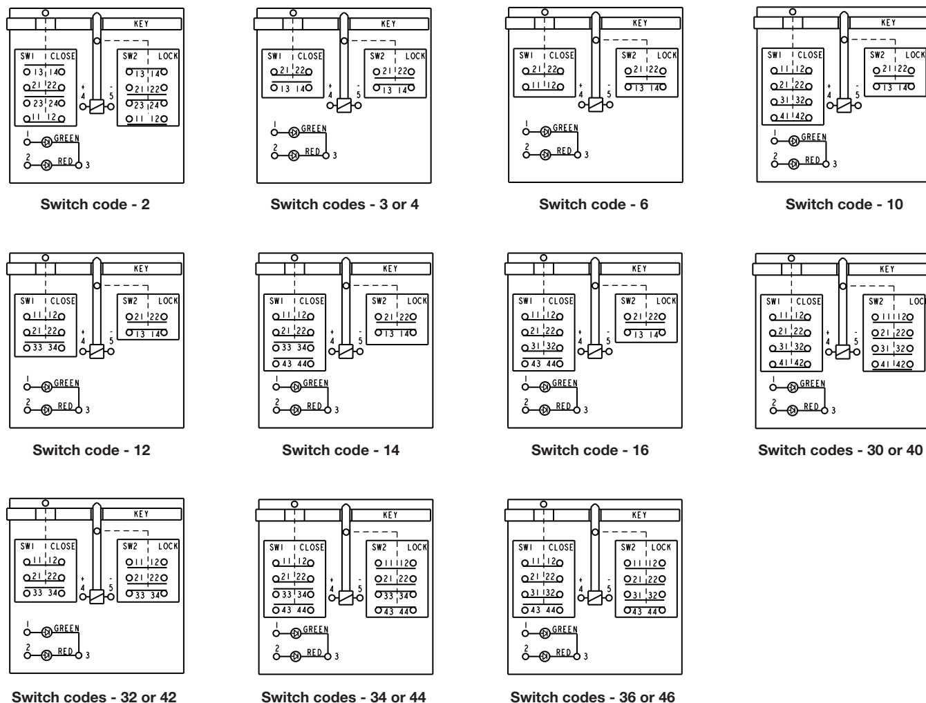
Figure 3. Circuit Diagrams for Body/Indicator Codes L or R, S or T Type Over-ride Codes
