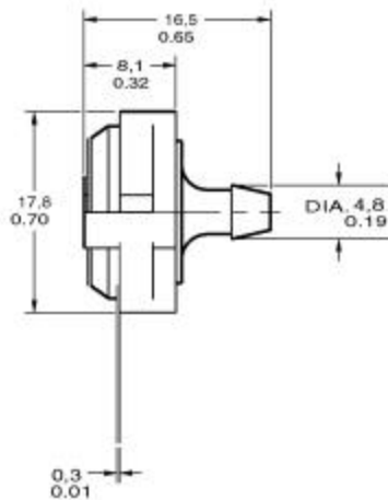
GBT Housing
