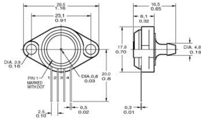
GBFS Housing
