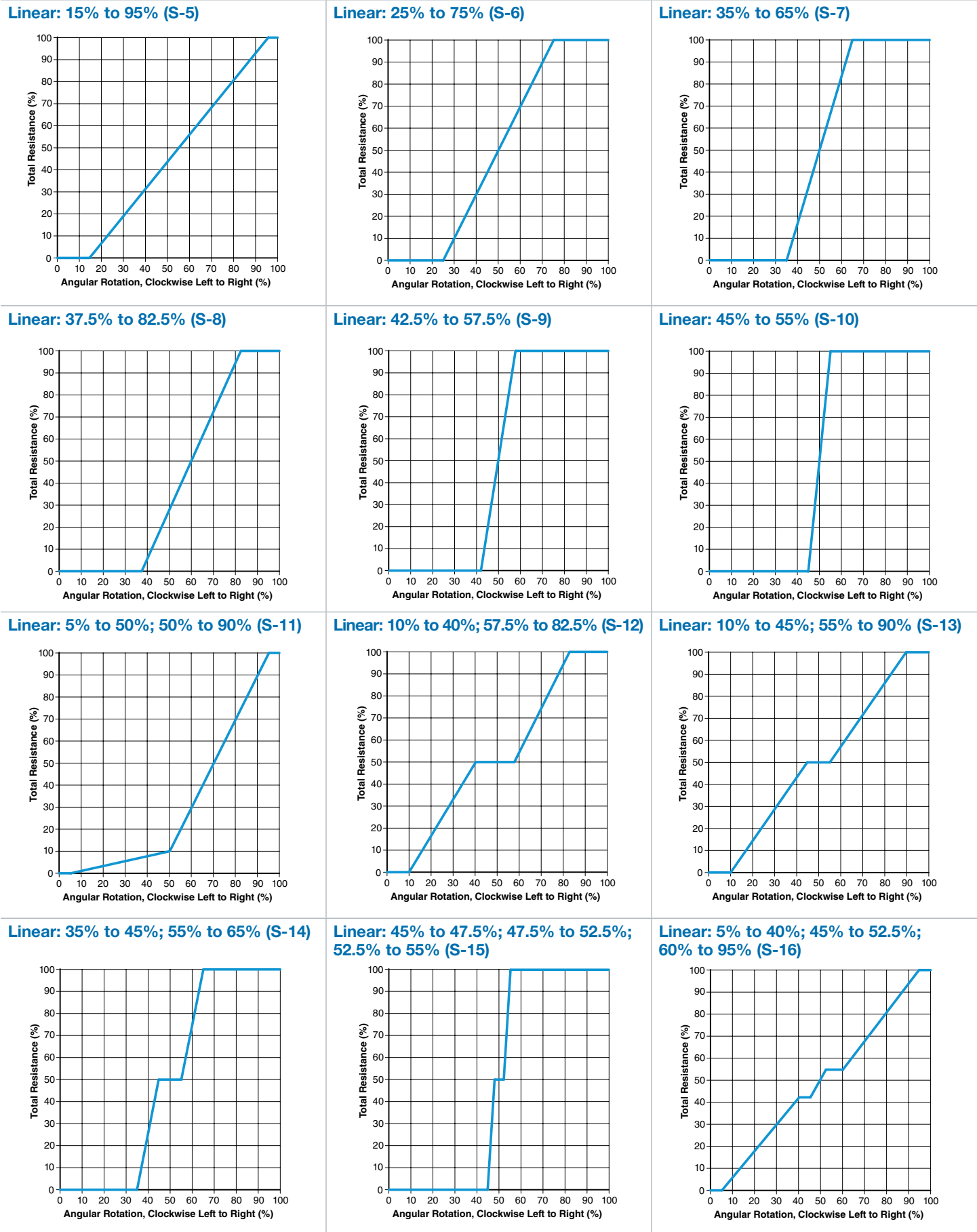
Figure 1. Electrical Taper Diagrams (continued)
