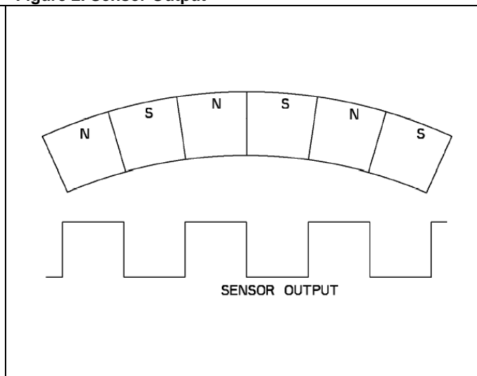
Figure 2. Sensor Output
