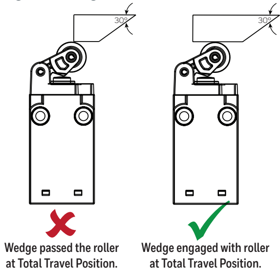
Figure 17. Wedge Actuation
