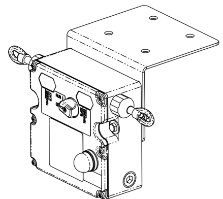
Figure 9. CPS-Bracket
