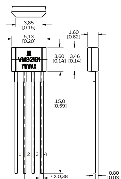
Figure 5. Dimensions and Product Marking (For reference only mm/[in])
