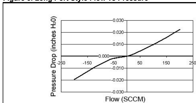
Figure 5. Long Port Style Flow vs Pressure
