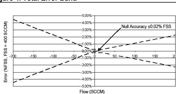
Figure 4. Total Error Band
