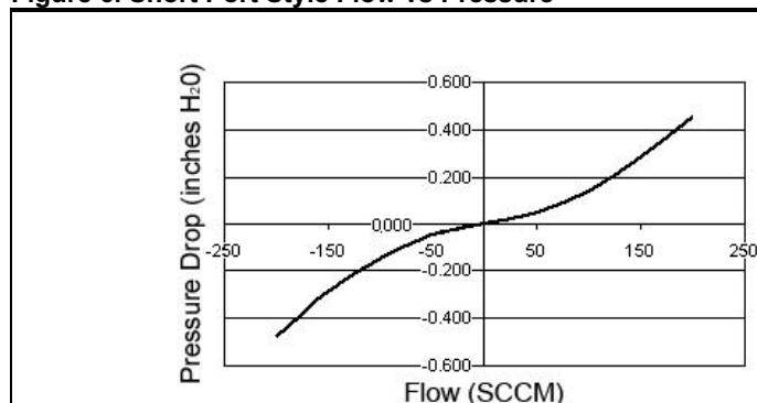
Figure 6. Short Port Style Flow vs Pressure
