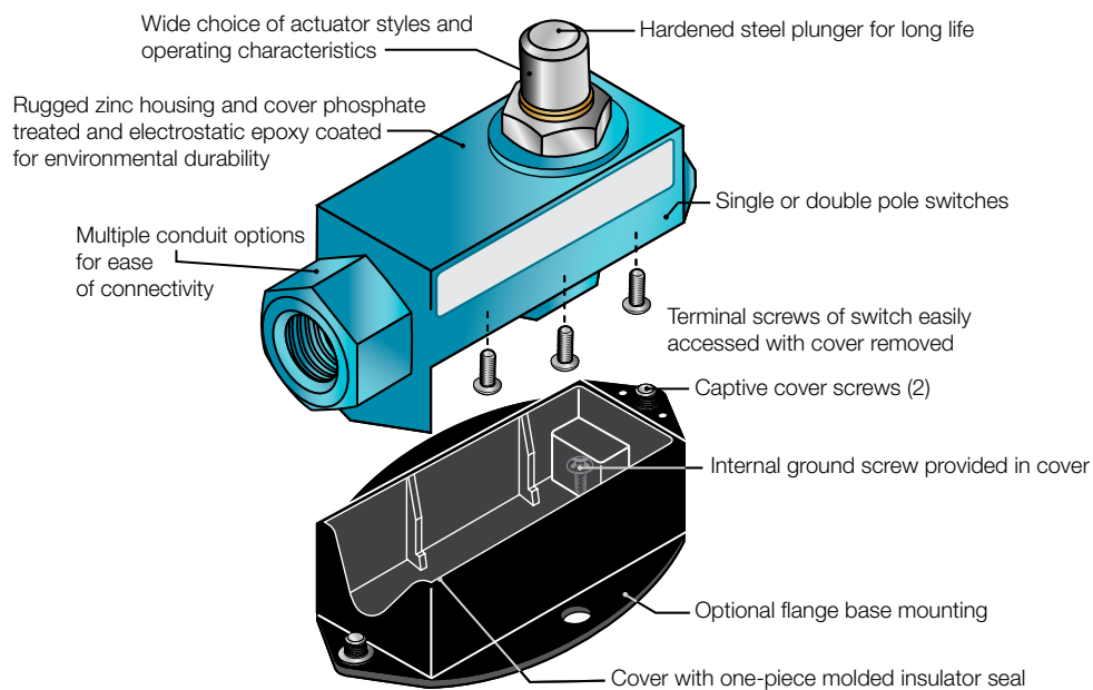
Figure 1B. V6 Flange mount without boot sealed actuator (typical)
