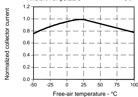
Fig. 6 Collector Current vs Ambient Temperature
