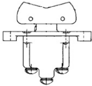
TP Series Rocker Switch, 2 pole, 3 position, Screw terminal, Above Panel Mounting
