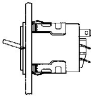
AML35 Series Paddle Switch, SPST, 2 position, Silver Contacts, 0.187 in x 0.02 in (Solder or Quick-Connect), 1 Lamp Circuit, Rectangle, Paddle, Snap-in Panel
