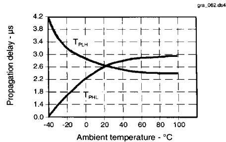
Fig. 2 Delay Time vs Temperature
