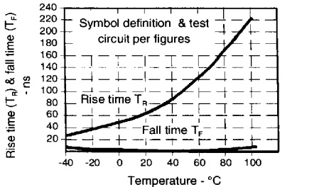
Fig. 1 Output Rise Time ( t_r ) and Output Fall Time ( t_f ) vs Temperature
