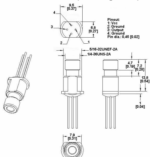
FIGURE 9. HFD3023-500-AAA (SMA Single Hole)
