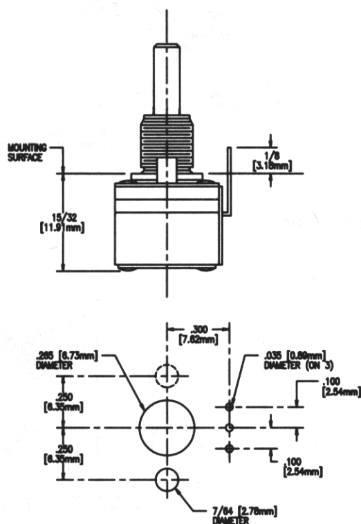
PC BOARD LAYOUT
