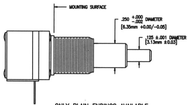
Figure 21 .125/.250 (3.18/6.35 mm) Diameter, Concentric Shafts
