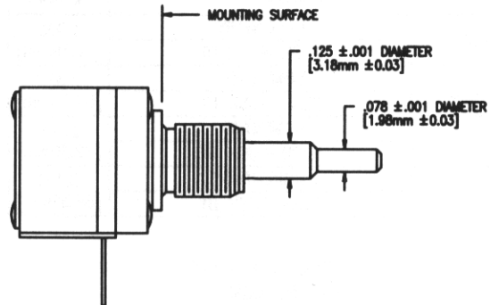
Figure 20 .078/.125 (1.98/3.18 mm) Diameter, Concentric Shafts
