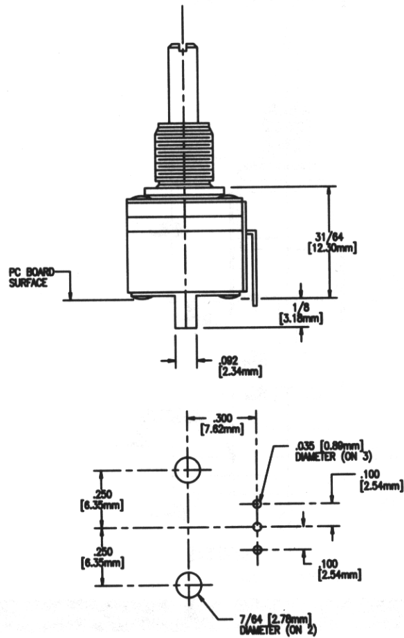
PC BOARD LAYOUT
