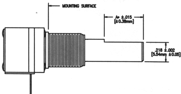
Figure 19 .250 (6.35mm) Diameter, Flatted Shaft
