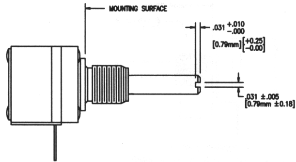
.125 ±.001 (3.18mm ±0.03) Diameter, Slotted Shaft
