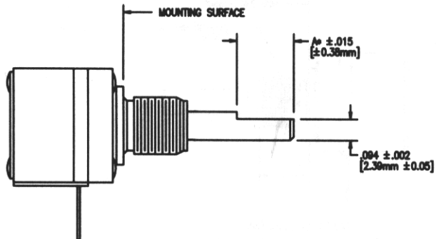
Figure 18 .125 ±.001 (3.18mm ±0.03) Diameter, Flatted Shaft
