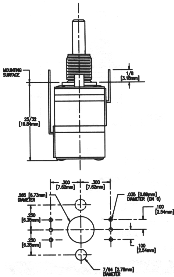
PC BOARD LAYOUT
