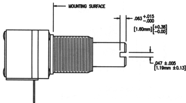
Figure 17 .250 +000/-.002 (6.35mm +0.00/-0.05) Diameter, Slotted Shaft
