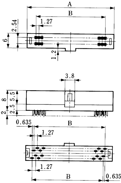
(40.60.80.100 contacts)
