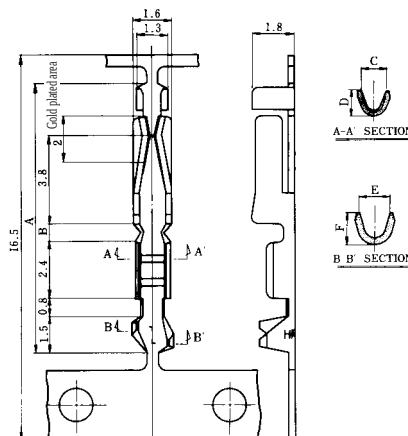
SCFC contact
