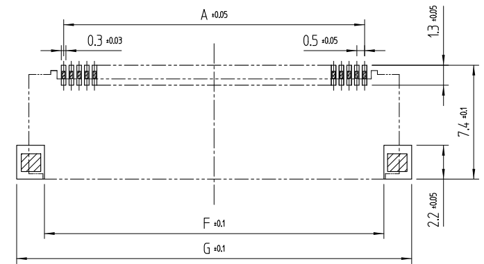
RECOMMENDED PCB LAND PATTERN (Non scale) (RECOMMENDED METAL MASK THICKNESS : t=0.12)
