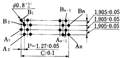
Mating Side
