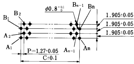
Mating Side
