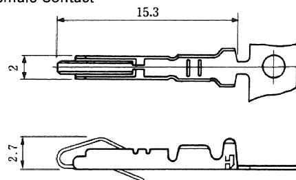
Female Contact
