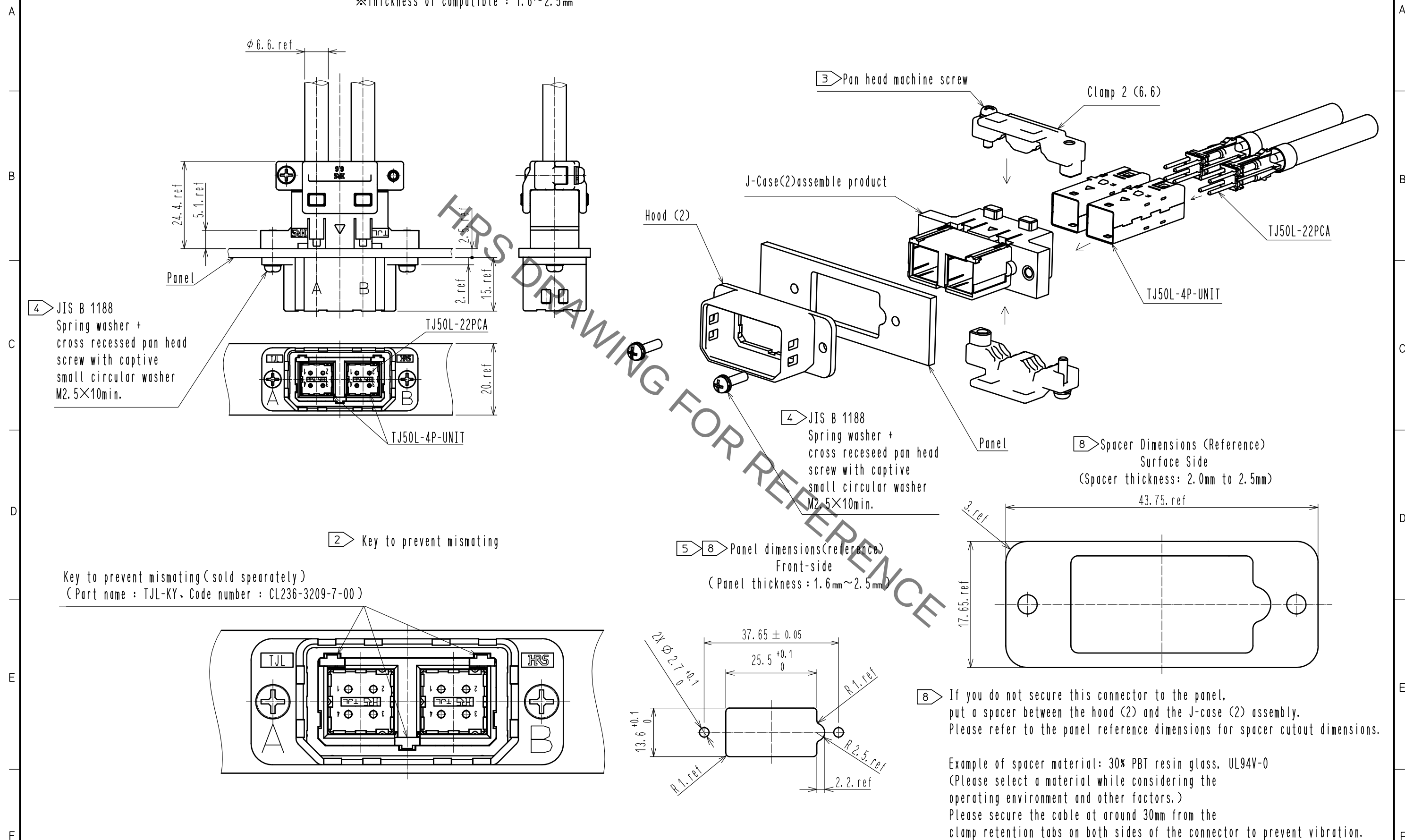
Mounted state drawing (Cable & Panel)(1:1)
