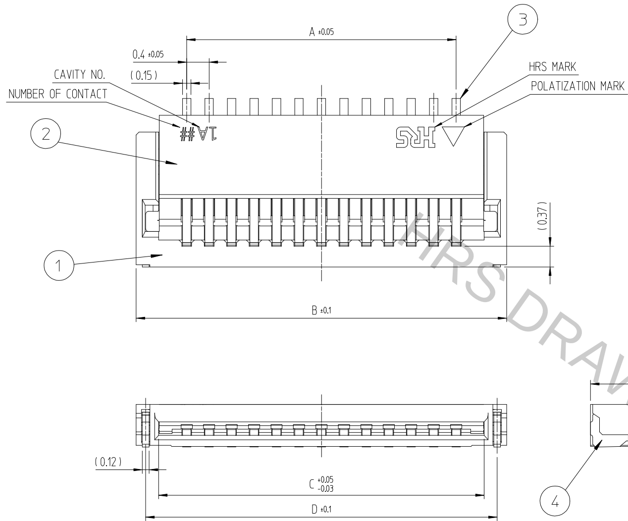
VIEW B (20:1)
