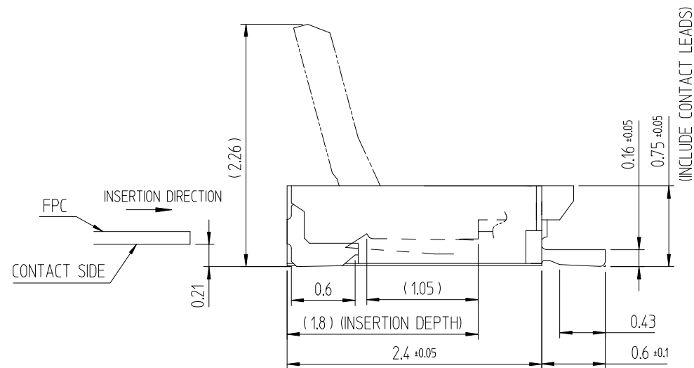
VIEW B (20:1)
