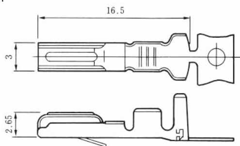
Male power terminal
