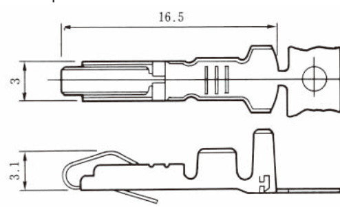
Female power terminal
