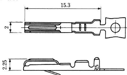
Male Contact
