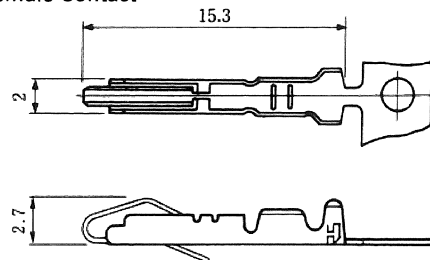
Female Contact
