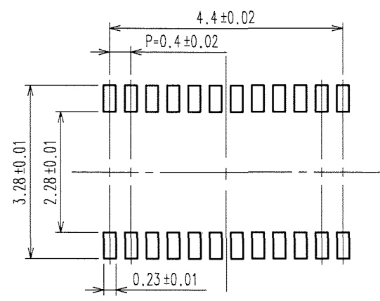
RECOMMENDED METAL MASK OPENING PATTERN
