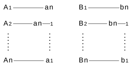
Connection of Cable 1
