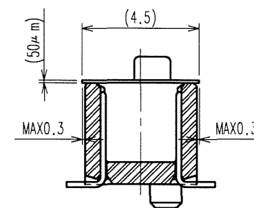
DETAIL OF TAPE FOR VACUUM PICKUP(5:1)
