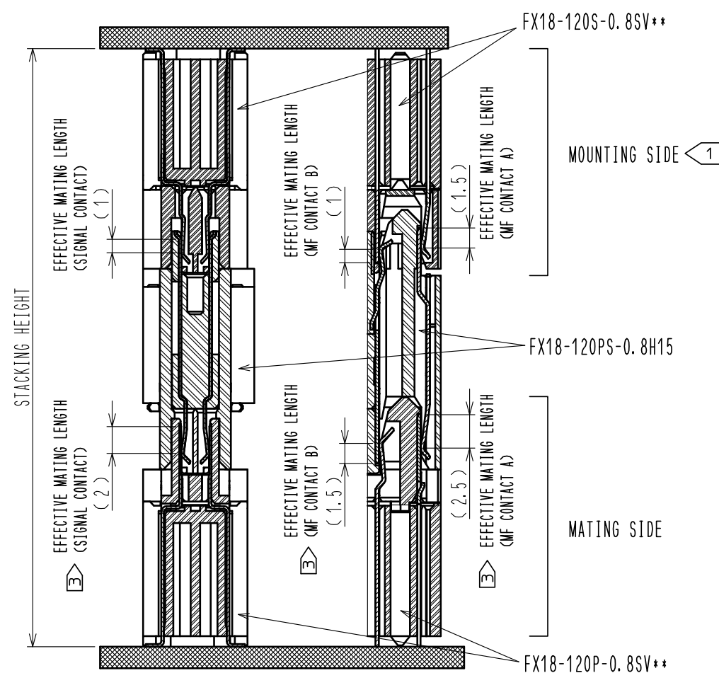
CROSS SECTION OF MATING(FREE)
