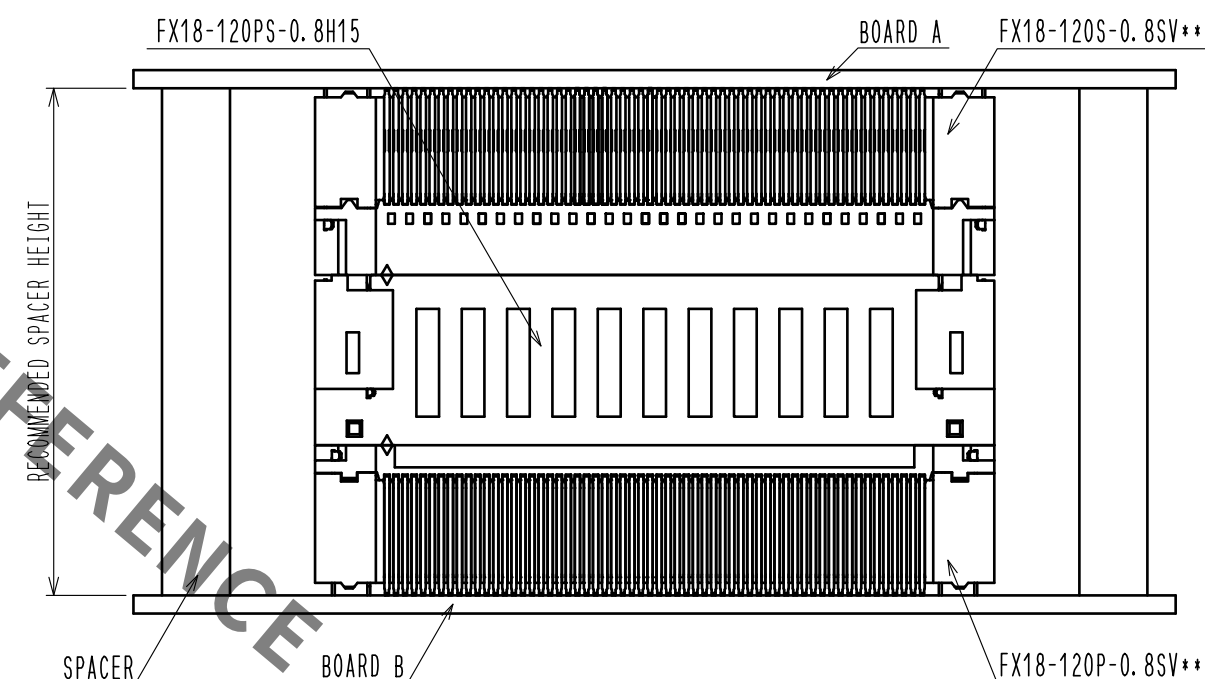
8 RECOMMENDED SPACER HEIGHT FOR EACH COMBINATION
