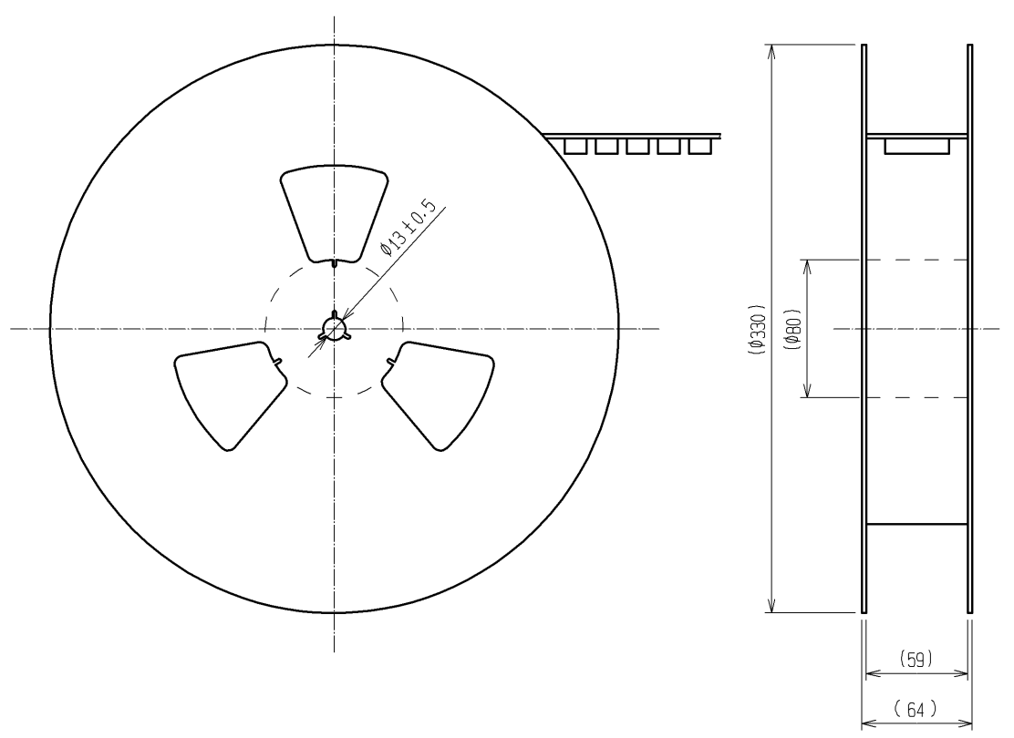
REELED DIMENSION(Free)
