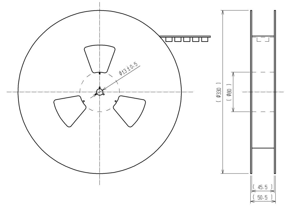
REELED DIMENSION(Free)
