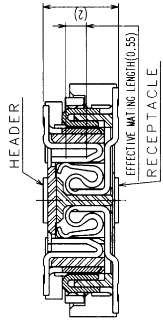
SIGNAL PORTION CROSS SECTION (10:1)
