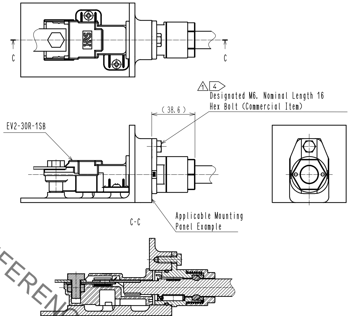
Mated Condition Diagram(1:2)
