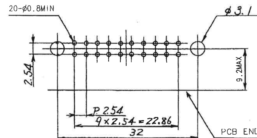
RECOMMENDED PC BOARD PATTERN
