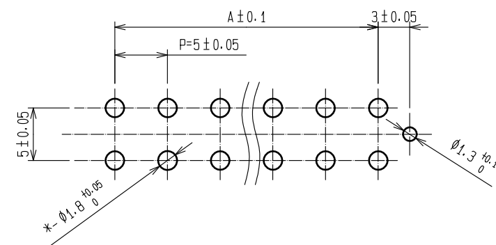
RECOMMENDED PCB LAYOUT ( t=1.6 \pm 0.1 )
