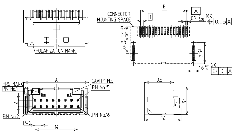
Recommended PCB Layout (t=1.6mm)
