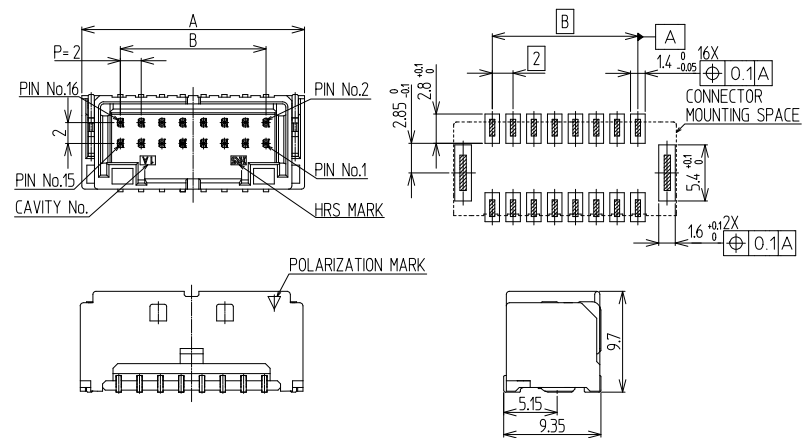
Recommended PCB Layout (t=1.6mm)
