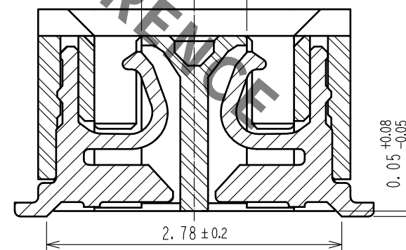
A-A (20:1) PICK AND PLACE AREA : 0.99 \pm 0.1
