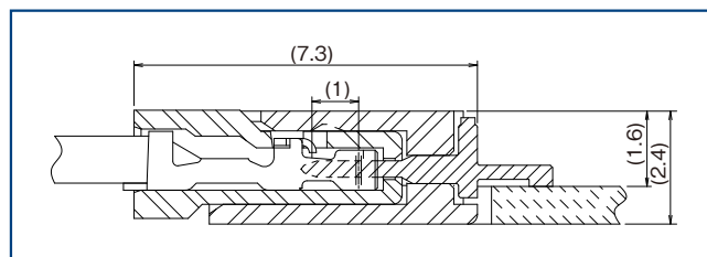
DF14H Offset Type Board Mounted Diagram
