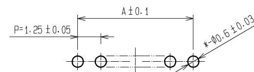
RECOMMENDED PATTERN
