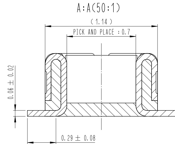
ENGAGEMENT FIGURE (50:1)
