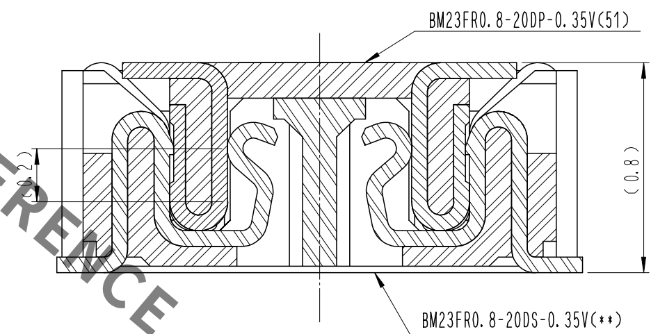
ENGAGEMENT FIGURE (50:1)
