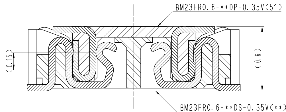
ENGAGEMENT FIGURE (50:1)
