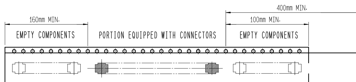
TRAILER
