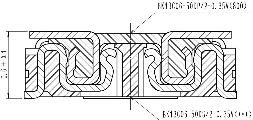
SIGNAL CONTACT
