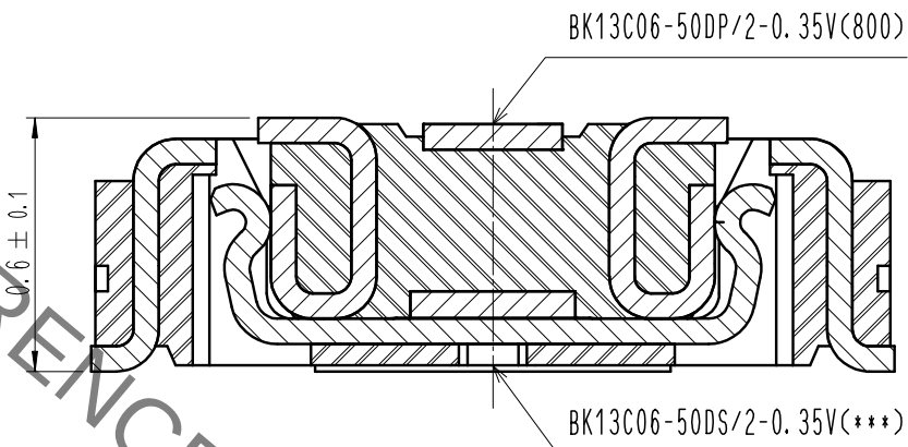
POWER CONTACT
