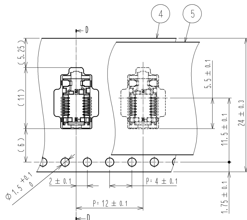
Dimensions of embossed carrier tape (Scale : FREE)
